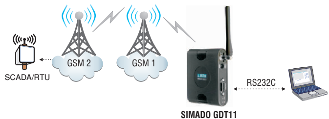
SIMADO GDT11 in Data Acquisition Application
